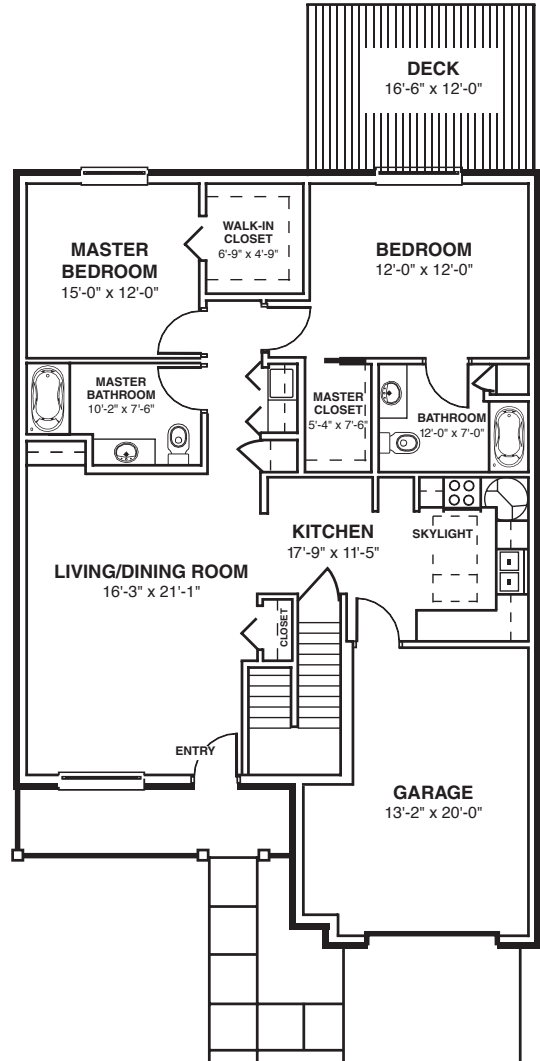
FLOOR PLAN
